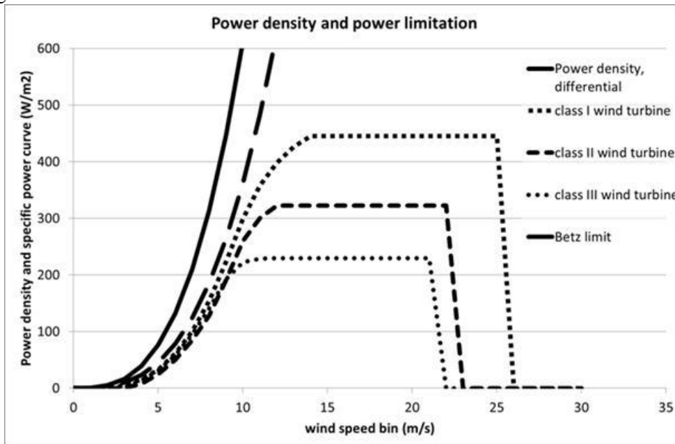
Fig. 3: Power density and power limitation
